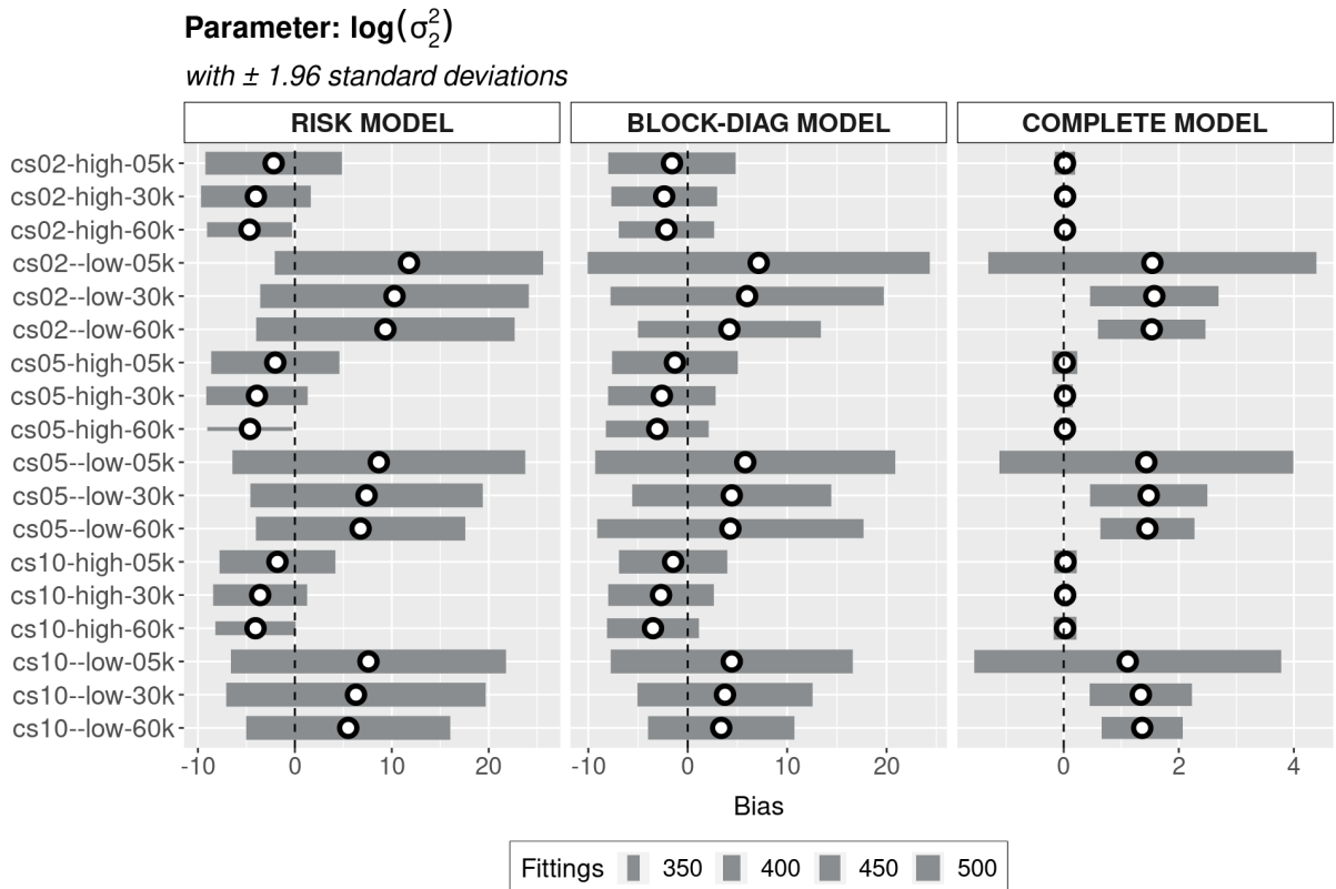
FIGURE 21 – PARAMETER \log(\sigma_2^2) BIAS WITH \pm 1.96 STANDARD DEVIATIONS
