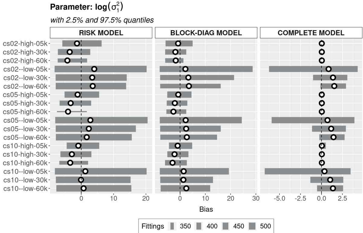
FIGURE 38 – PARAMETER \log(\sigma_1^2) BIAS WITH 2.5% AND 97.5% QUANTILES
