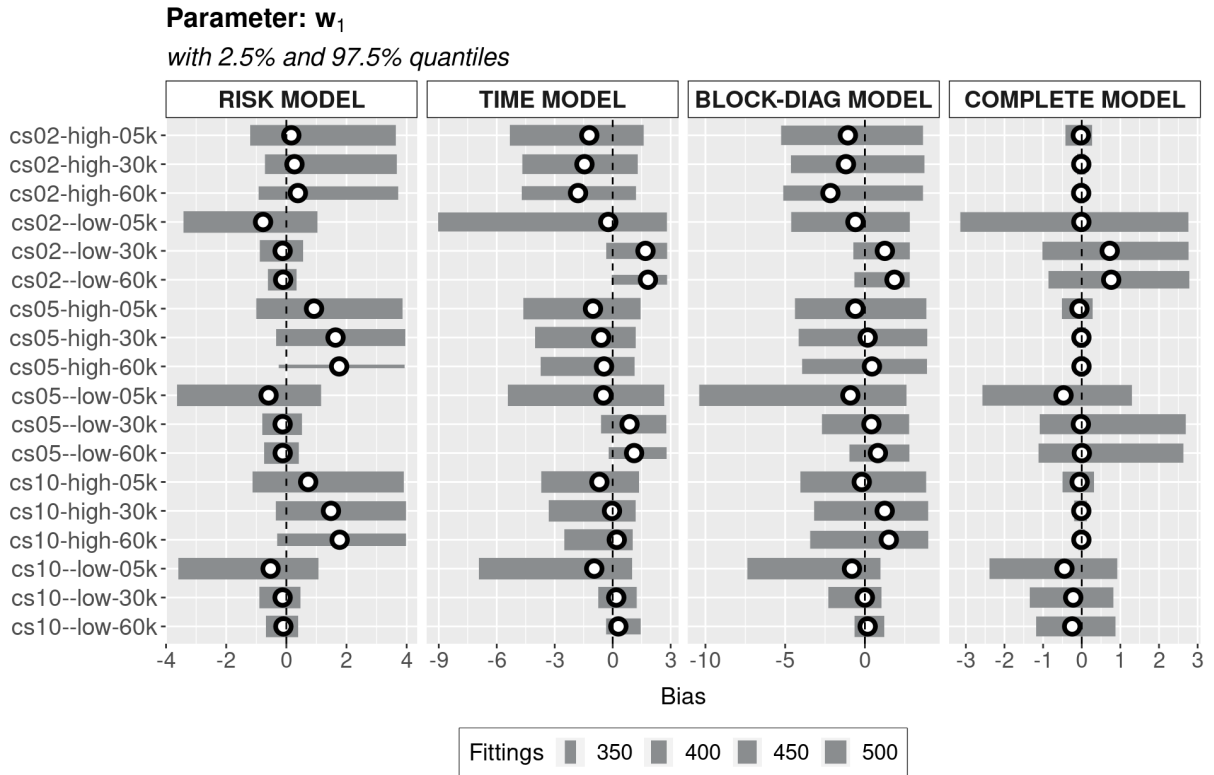
FIGURE 36 – PARAMETER w_1 BIAS WITH 2.5% AND 97.5% QUANTILES
