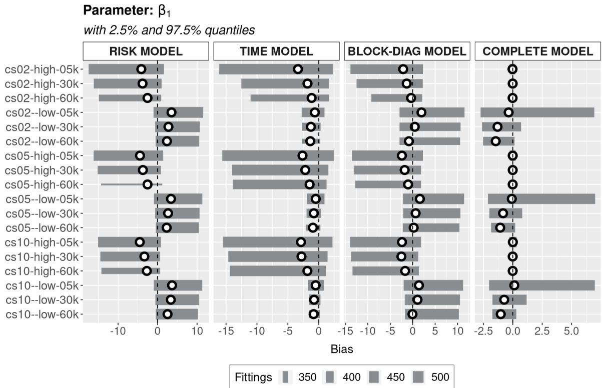
FIGURE 32 – PARAMETER \beta_1 BIAS WITH 2.5% AND 97.5% QUANTILES
