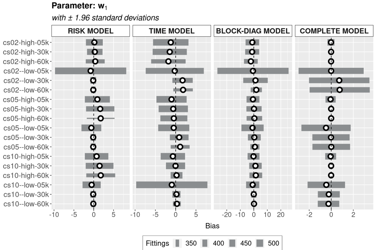
FIGURE 18 – PARAMETER w_1 BIAS WITH \pm 1.96 STANDARD DEVIATIONS
