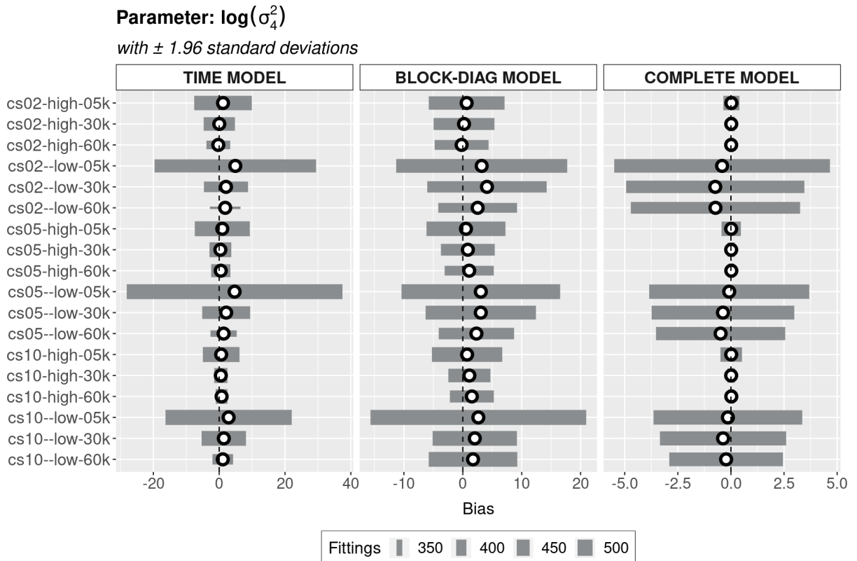
FIGURE 23 – PARAMETER \log(\sigma_4^2) BIAS WITH \pm 1.96 STANDARD DEVIATIONS
