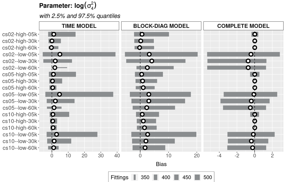
FIGURE 41 – PARAMETER \log(\sigma_4^2) BIAS WITH 2.5% AND 97.5% QUANTILES
