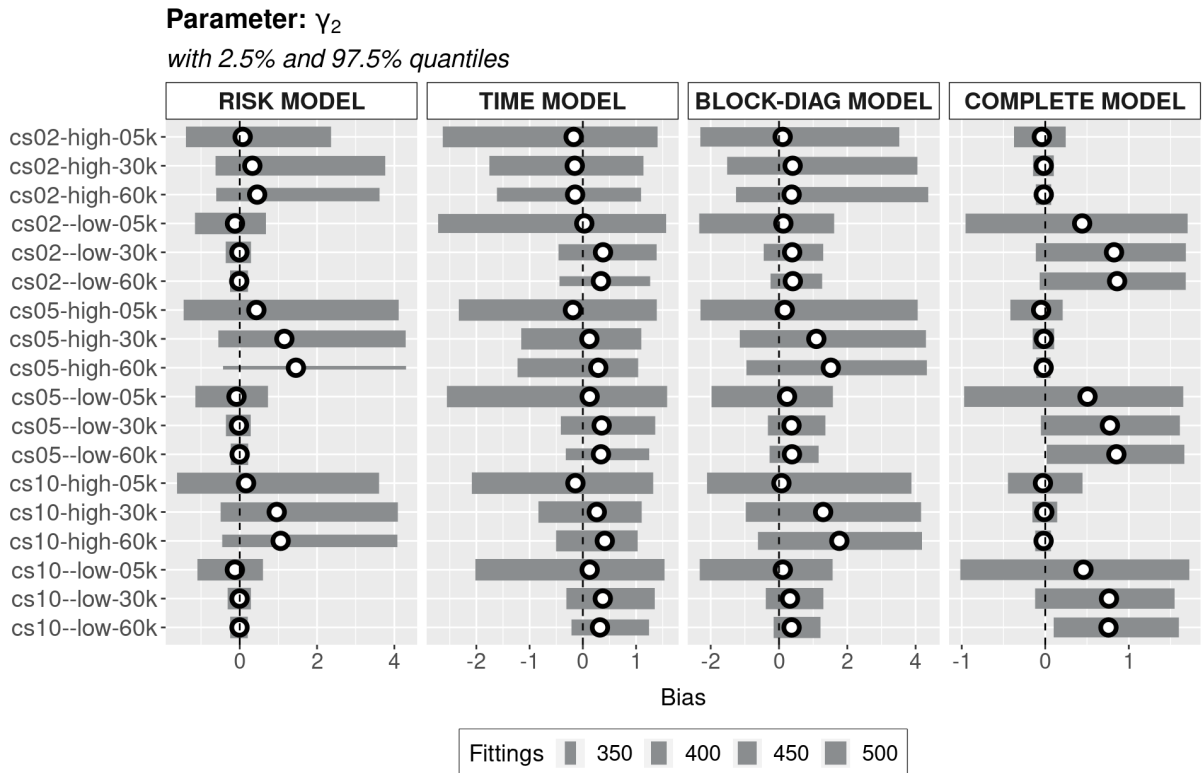
FIGURE 35 – PARAMETER \gamma_2 BIAS WITH 2.5% AND 97.5% QUANTILES
