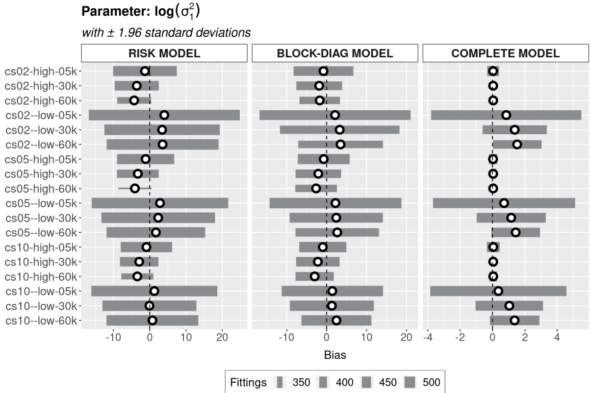
FIGURE 20 – PARAMETER \log(\sigma_1^2) BIAS WITH \pm 1.96 STANDARD DEVIATIONS
