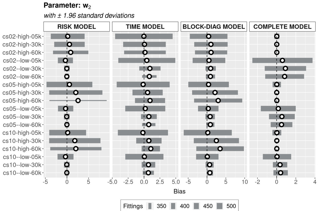
FIGURE 19 – PARAMETER w_2 BIAS WITH \pm 1.96 STANDARD DEVIATIONS
