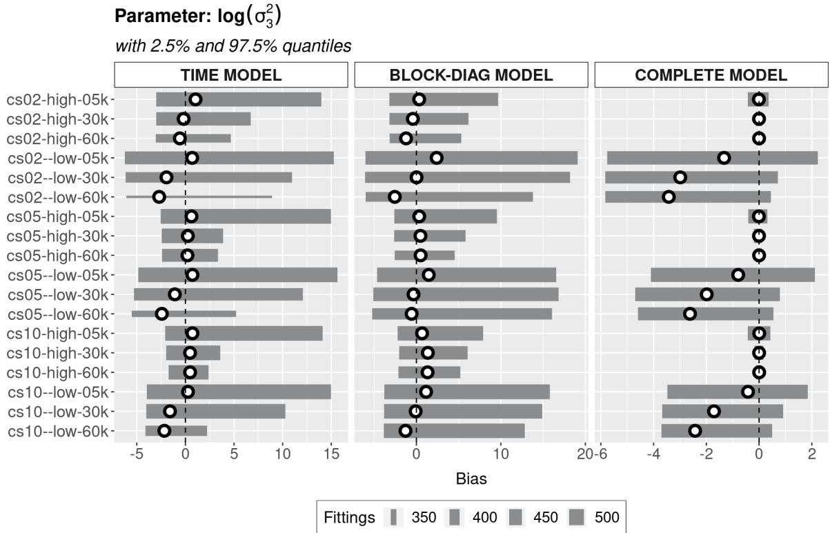
FIGURE 40 – PARAMETER \log(\sigma_3^2) BIAS WITH 2.5% AND 97.5% QUANTILES
