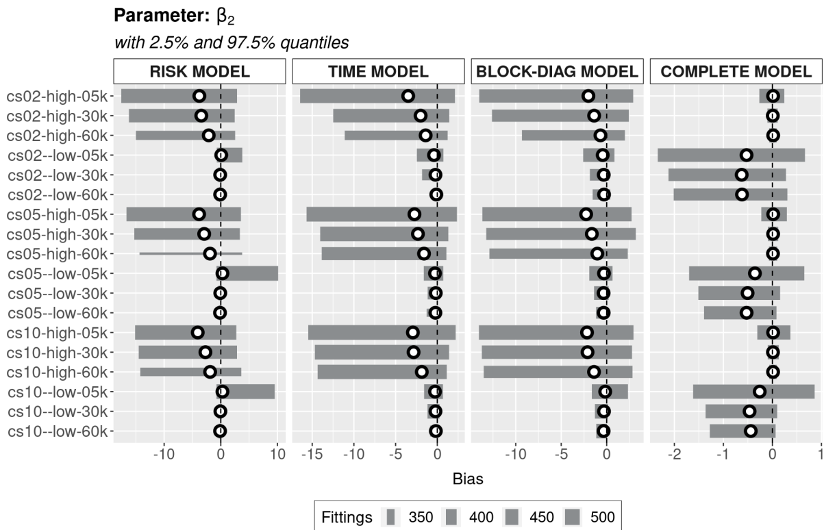
FIGURE 33 – PARAMETER \beta_2 BIAS WITH 2.5% AND 97.5% QUANTILES
