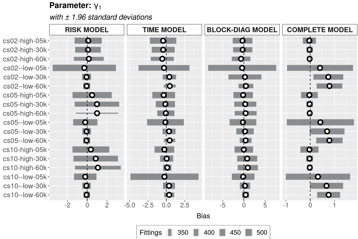
FIGURE 16 – PARAMETER \gamma_1 BIAS WITH \pm 1.96 STANDARD DEVIATIONS
