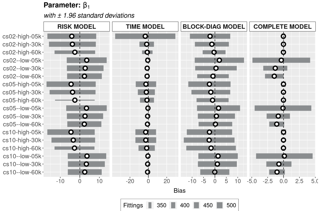
FIGURE 14 – PARAMETER \beta_1 BIAS WITH \pm 1.96 STANDARD DEVIATIONS
