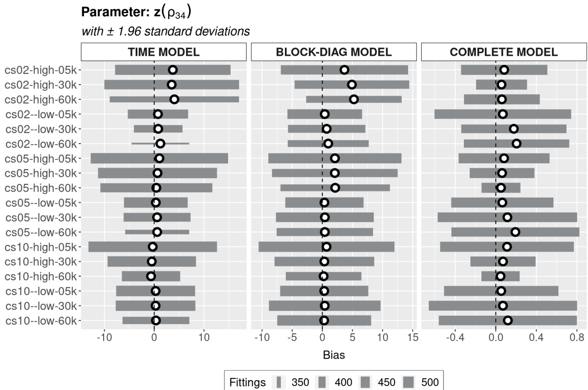
FIGURE 25 – PARAMETER z(\rho_{34}) BIAS WITH \pm 1.96 STANDARD DEVIATIONS
