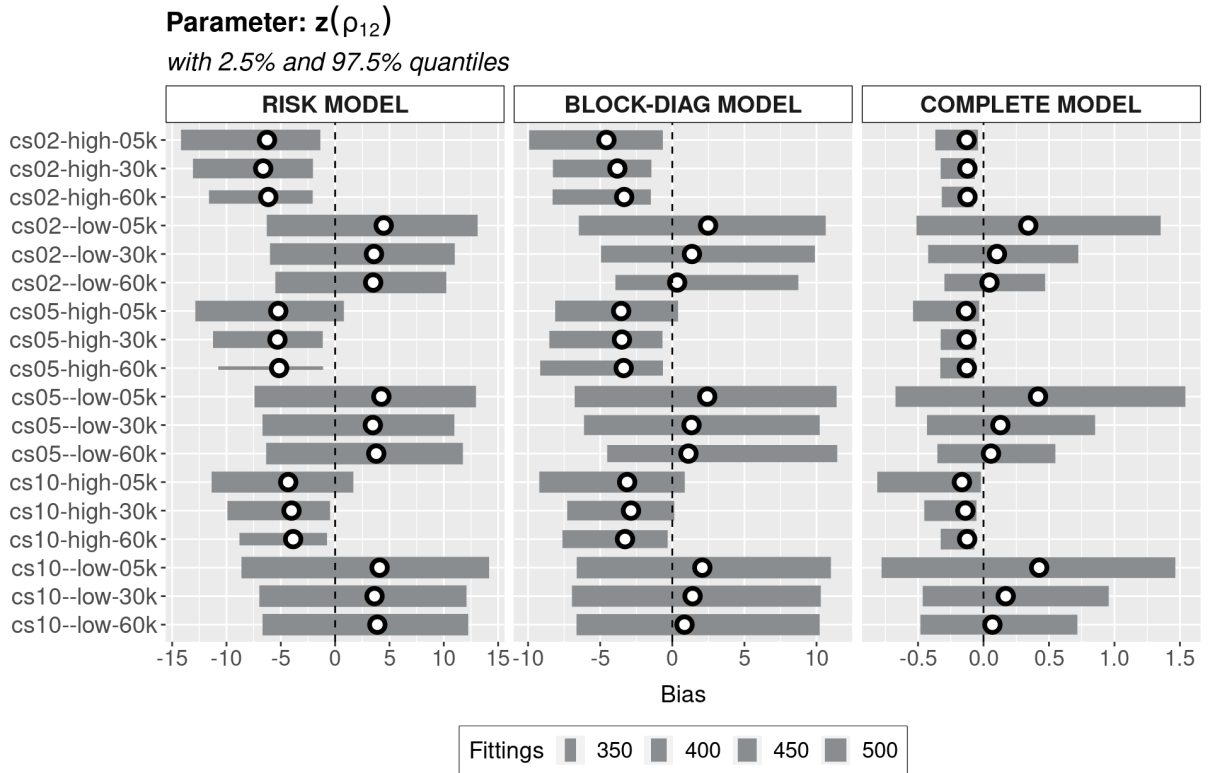
FIGURE 42 – PARAMETER z(\rho_{12}) BIAS WITH 2.5% AND 97.5% QUANTILES
