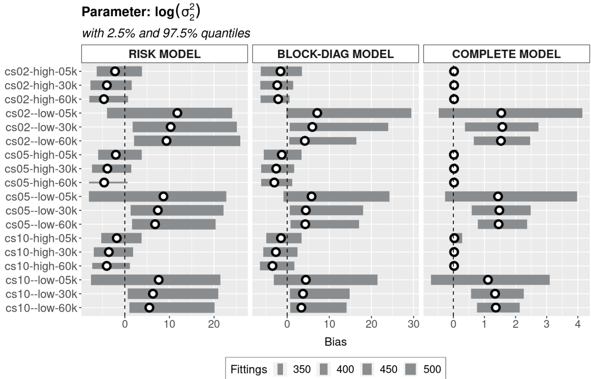
FIGURE 39 – PARAMETER \log(\sigma_2^2) BIAS WITH 2.5% AND 97.5% QUANTILES
