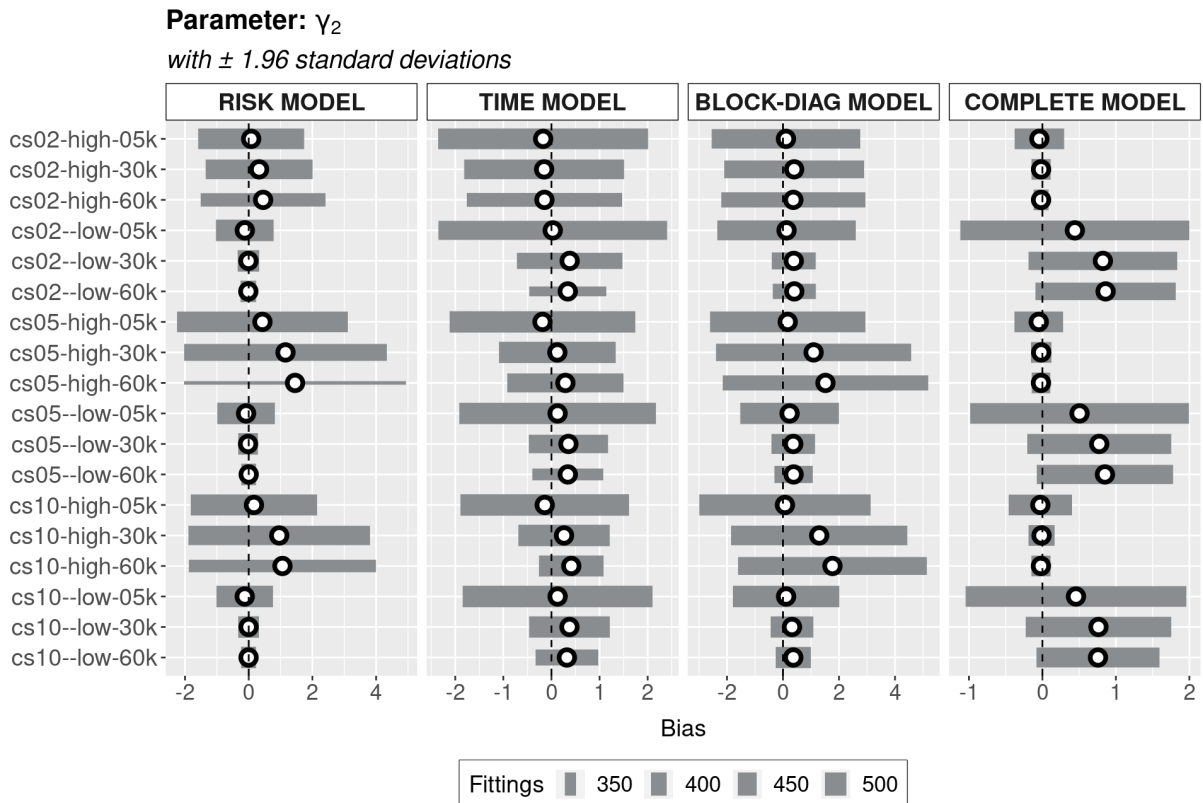
FIGURE 17 – PARAMETER \gamma_2 BIAS WITH \pm 1.96 STANDARD DEVIATIONS
