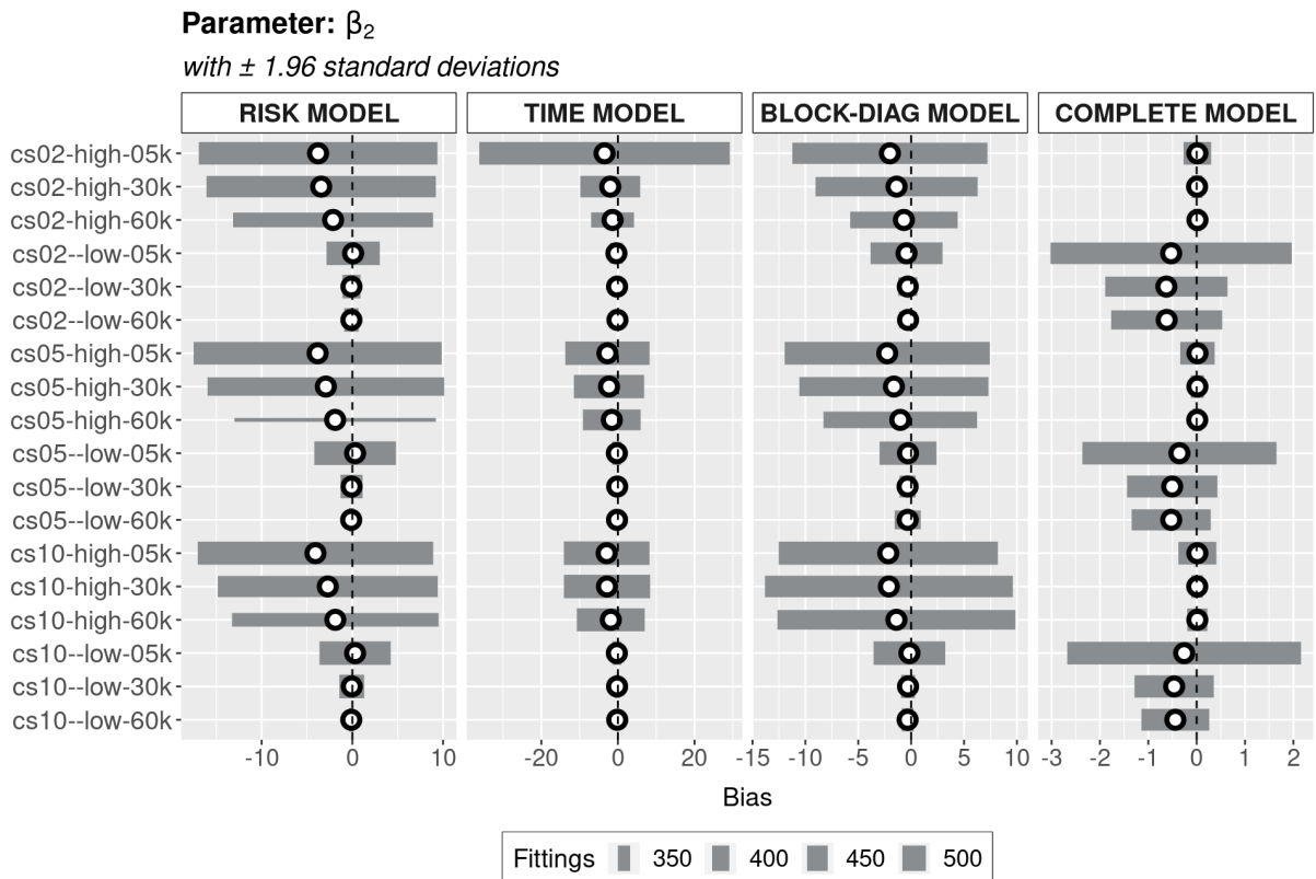
FIGURE 15 – PARAMETER \beta_2 BIAS WITH \pm 1.96 STANDARD DEVIATIONS
