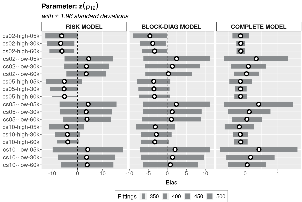
FIGURE 24 – PARAMETER z(\rho_{12}) BIAS WITH \pm 1.96 STANDARD DEVIATIONS
