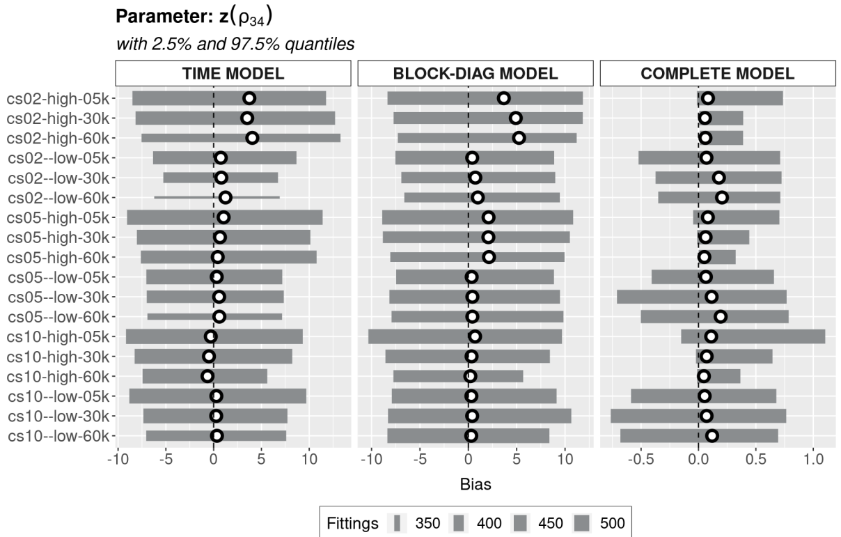
FIGURE 43 – PARAMETER z(\rho_{34}) BIAS WITH 2.5% AND 97.5% QUANTILES
