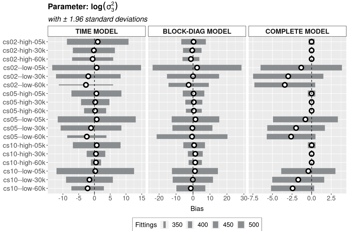
FIGURE 22 – PARAMETER \log(\sigma_3^2) BIAS WITH \pm 1.96 STANDARD DEVIATIONS
