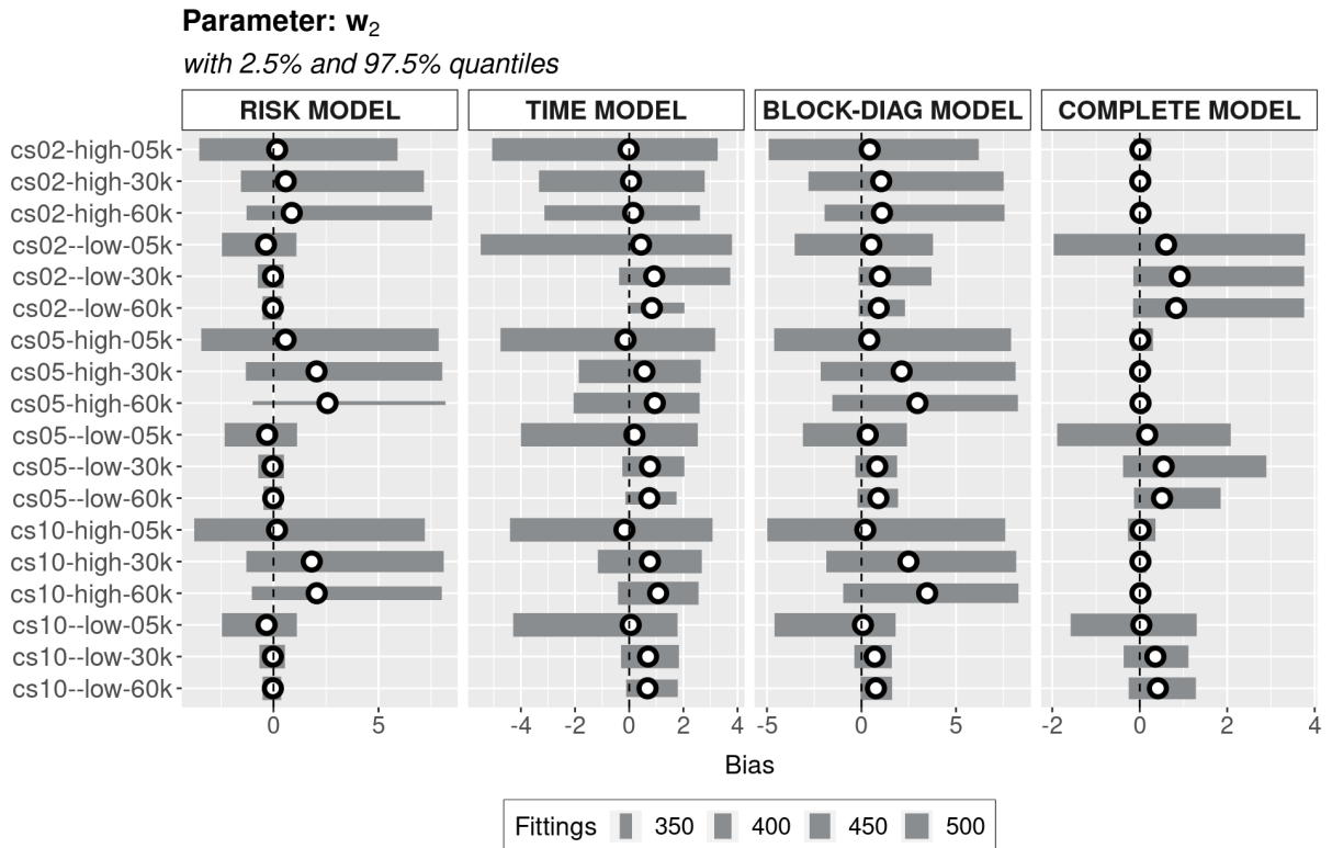
FIGURE 37 – PARAMETER w_2 BIAS WITH 2.5% AND 97.5% QUANTILES
