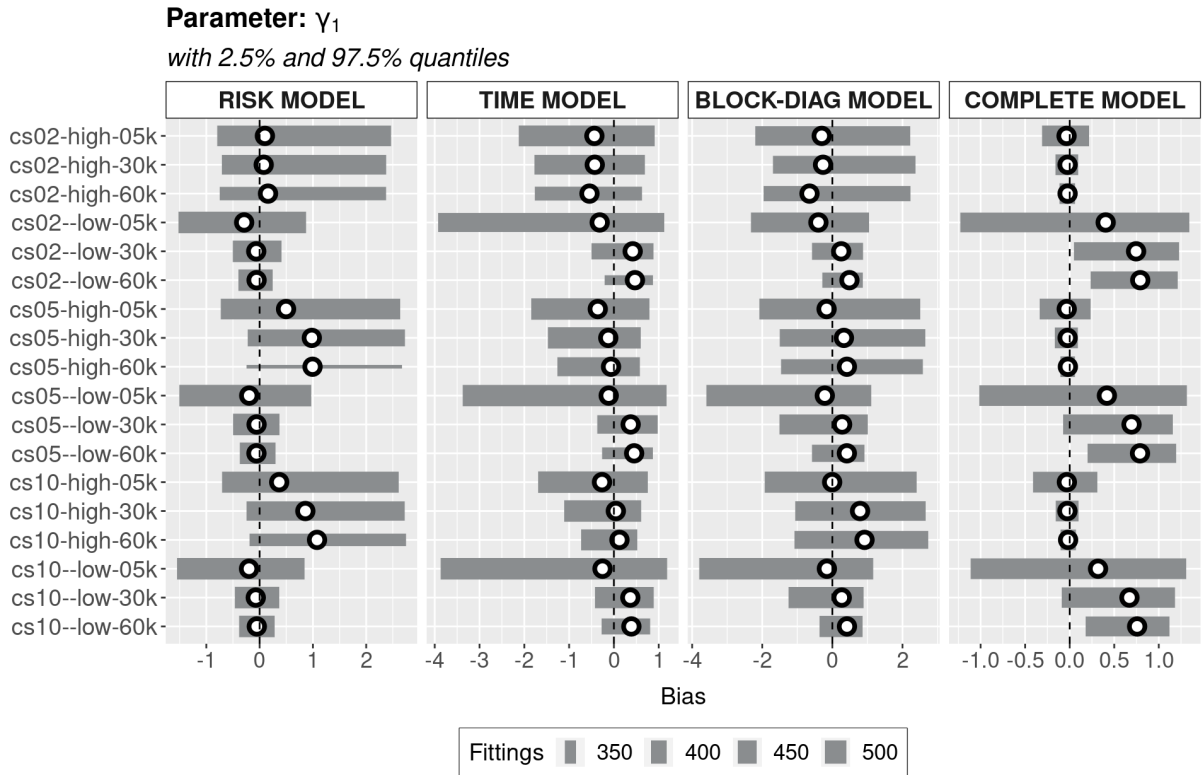
FIGURE 34 – PARAMETER \gamma_1 BIAS WITH 2.5% AND 97.5% QUANTILES
